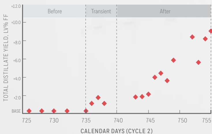
Process enhancement impact on distillate yields
